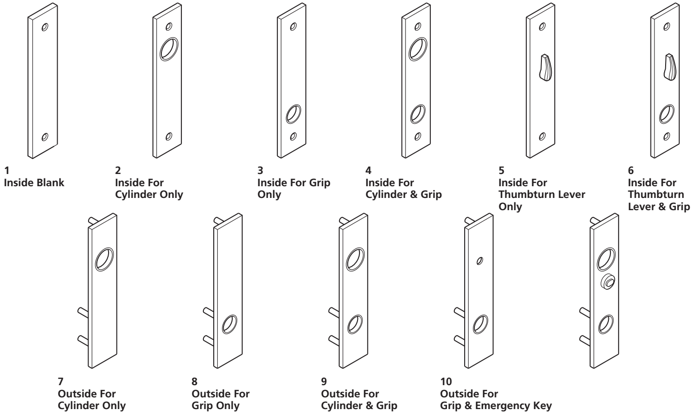
8-1/2" x 1-3/4" Cast (Specify Finish)
