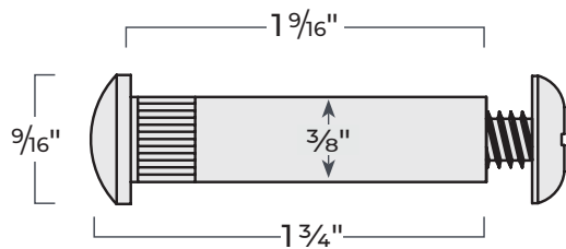
FDTB 3/8"
