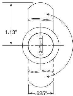
383257 (Door Lock)
