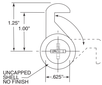
4706-175 (Security Lock) CAT Key 118
