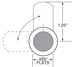
314370-22 (Knob Latch)
