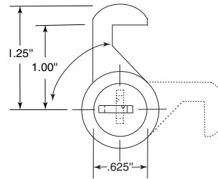
4706-175 (Security Lock) CAT Key 118
