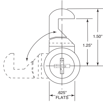
314370-22 (Knob Latch)
