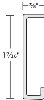
INSTALLED VIEW
