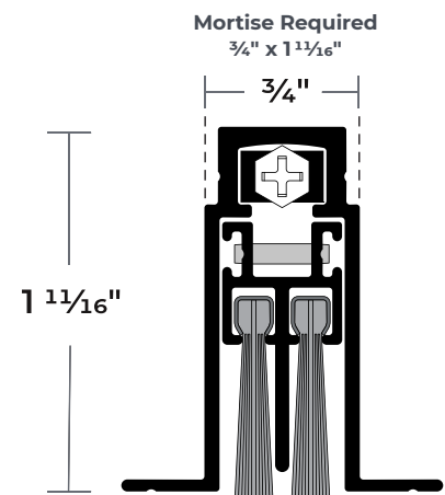
683A Nylon Brush Seal with EPDM Rubber Insert
