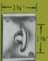
125MA: Brass, Bronze, Aluminum Extruded plate, Forged knob Finishes: 3, 4, 10, 26, 26D, 28 Regularly furnished with 3/16" Spindle.
