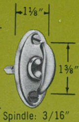
125: Brass, Bronze and aluminum Wrought Plate, Forged knob Finishes: 3, 4, 10, 26, 26D, 28 Regularly furnished with 3/16" Spindle.
